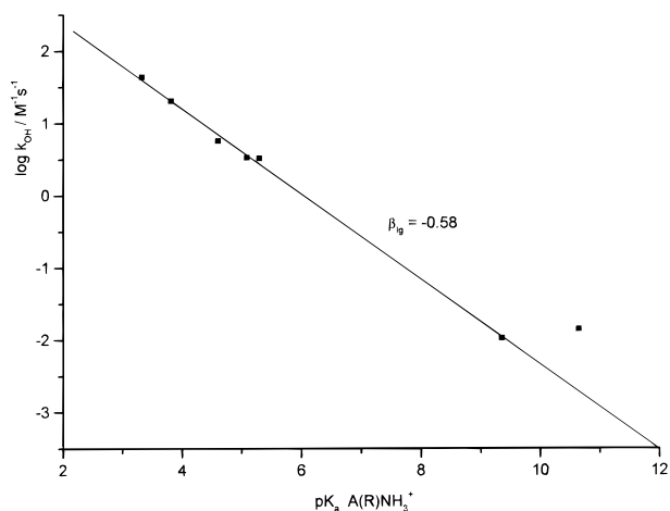
Figure 5. Brønsted plot of the second-order rate constants for the alkaline hydrolysis of N -aryl-substituted \beta -sultams against the \text{pK}_a 's of the corresponding anilinium ions at 30 °C and I = 1.0 M (KCl). Also shown is the extrapolated line for two N -alkyl- \beta -sultams.
