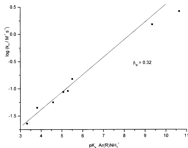
Figure 6. Brønsted plot of the second-order rate constants for the acid-catalyzed hydrolysis of N -aryl-substituted \beta -sultams against the pK_a 's of the corresponding anilinium ions at 30 °C and I = 1.0 M (KCl). Also shown is the extrapolated line for two N -alkyl- \beta -sultams.
