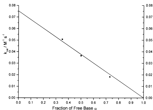
Figure 8. Plot of the catalytic coefficient k_{cat} against the fraction of free base \alpha in the formate/formic acid buffer catalyzed hydrolysis of N -benzyl- \beta -sultam at 30 °C and I = 1.0 M (KCl).
